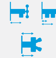
Stop Tap Dimensions (mm)
