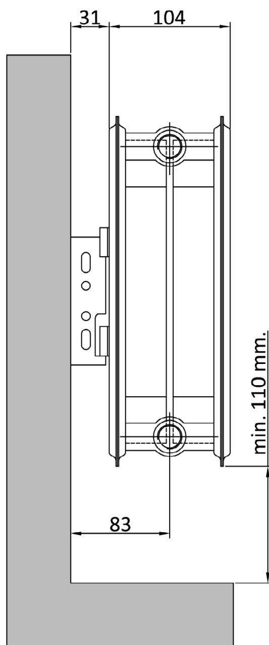
TIP / TYPE:22-PKKP
