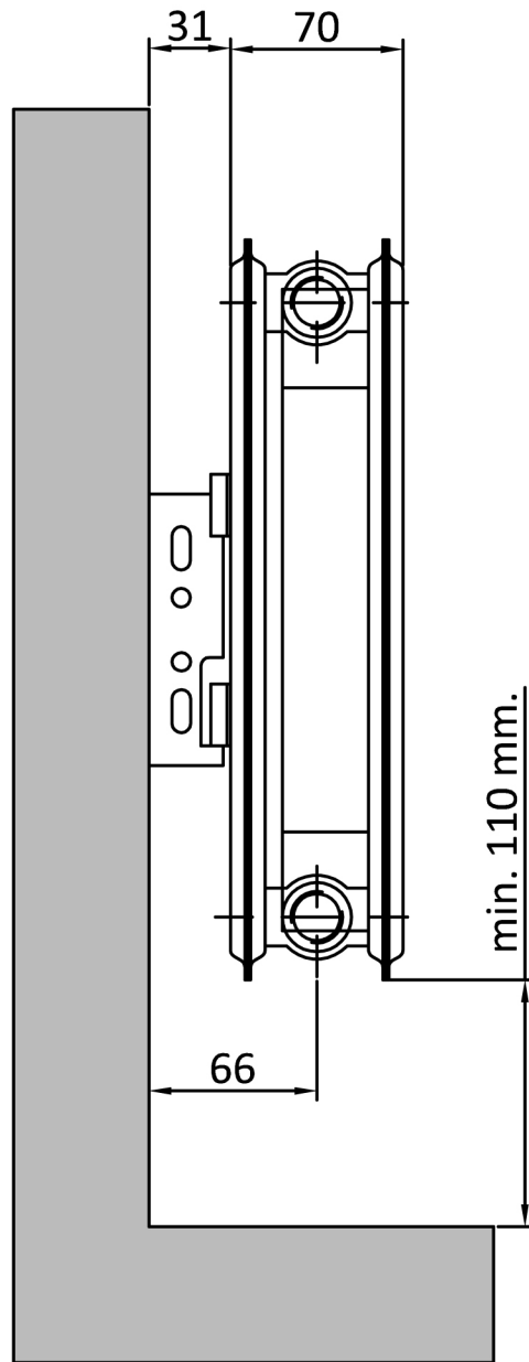
TIP / TYPE:21-PKP
