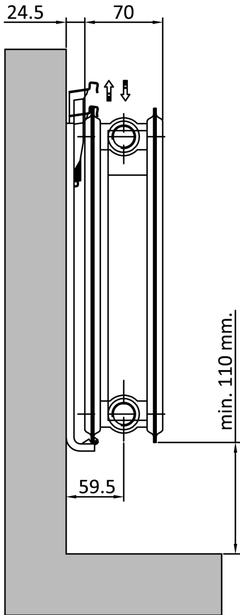
TIP / TYPE:21-PKP
